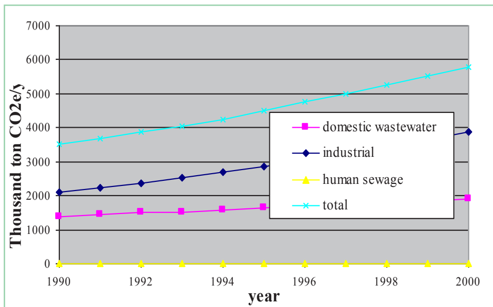
Figure (II.13): Total emissions (1000 ton CO 2 e/year) from wastewater handling.
