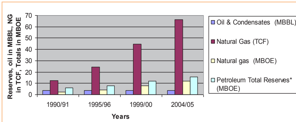
Figure (I.7): Crude oil and natural gas reserves in Egypt, 1990 to 2005. 5
