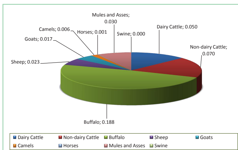
Figure (II.8): Total CH 4 emissions (Mt) from livestock categories due to enteric fermentation, 2000.
