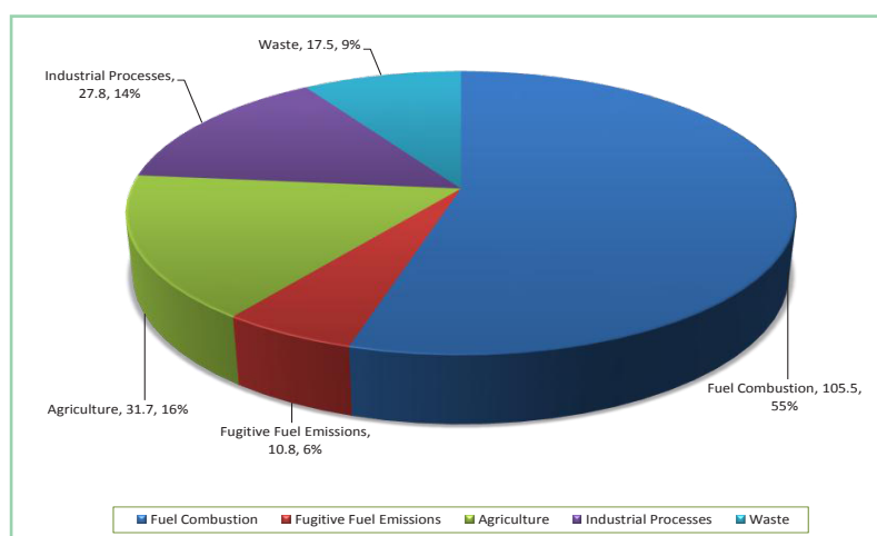
Figure (II.2): Egypt's GHG emissions by sector for the year 2000, in Mt CO 2 e.
