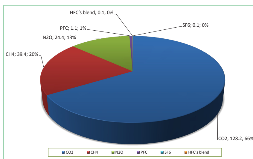
Figure (II.1): Egypt's GHG emissions by gas type for the year 2000 in Mt CO 2 e.
