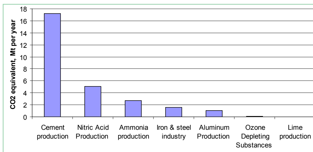
Figure (II.7): GHG emissions by different industrial sectors, according to gas type, 2000.
