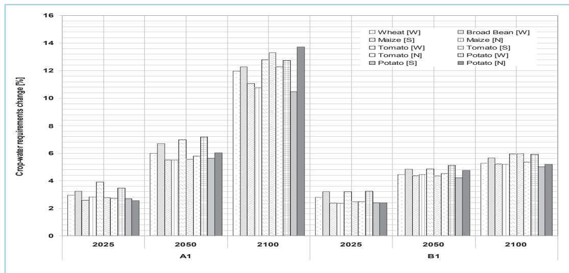
Figure (IV.4): Change between current and future values (for years 2025, 2050 and 2100) at national level seasonal crop-water requirements of some field and vegetable major crops (Attaher and Medany, 2008).
