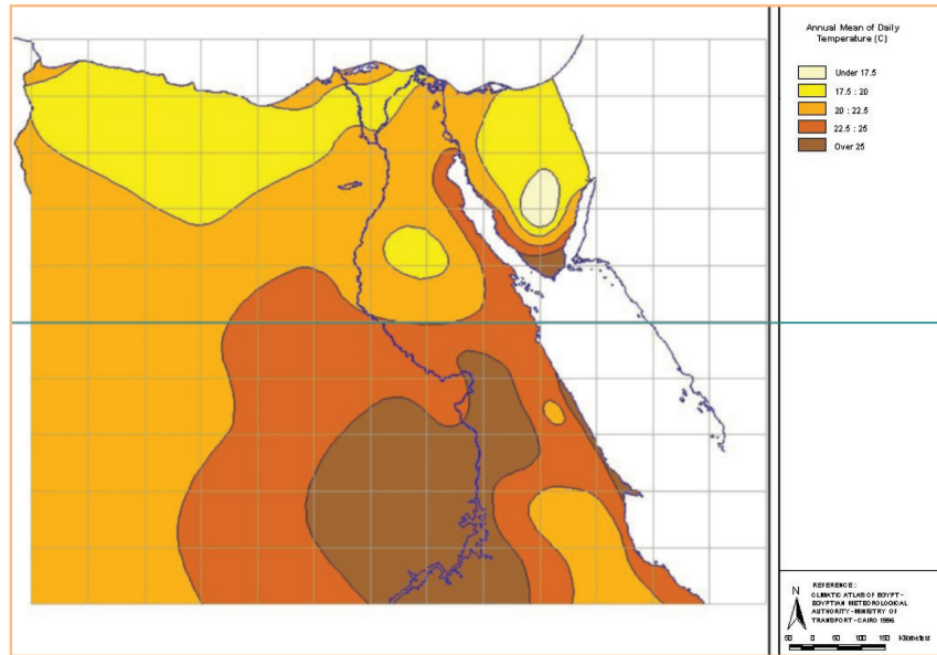
Figure (I.2): Average annual mean of daily temperature (°C). 2
