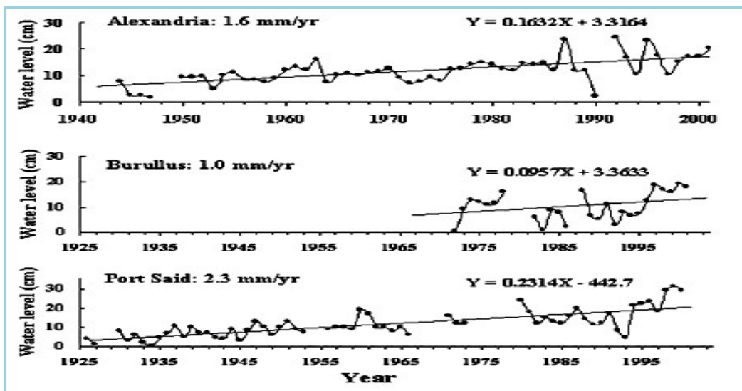
Figure (IV.6): Long term Sea-Level rise based on mean annual sea levels measured by tide gauges located at Alexandria, Burullus and Port Said (Frihy, 2003).
