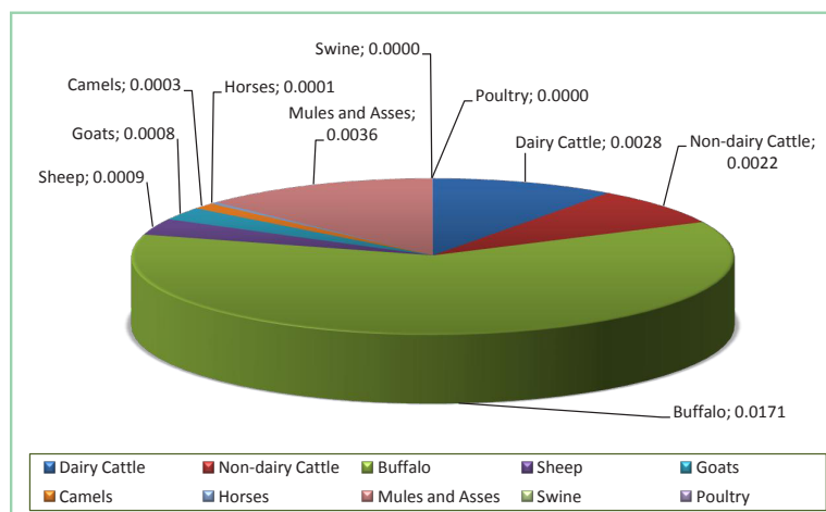
Figure (II.9): Total CH 4 emissions (Mt) from livestock categories due to manure management, 2000.
