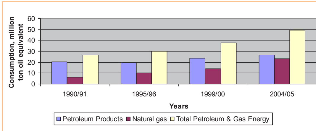
Figure (I.9): Consumption of petroleum products and natural gas in Mt, 1990/91 to 2005/06. 5
