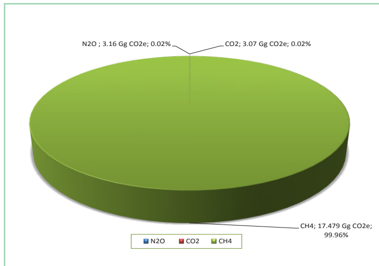
Figure (II.10): Emissions and relative weight of GHG for the waste sector, 2000.
