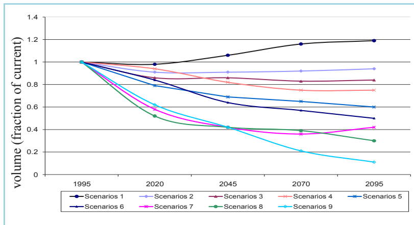
Figure (IV.1): Scenarios of changes in Nile flows (Strezpek et al., 2001).
