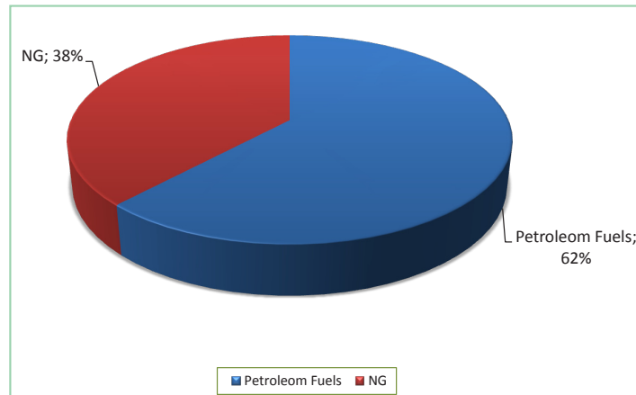
Figure (II.4): GHGs emissions from petroleum fuels and NG, 2000/01.
