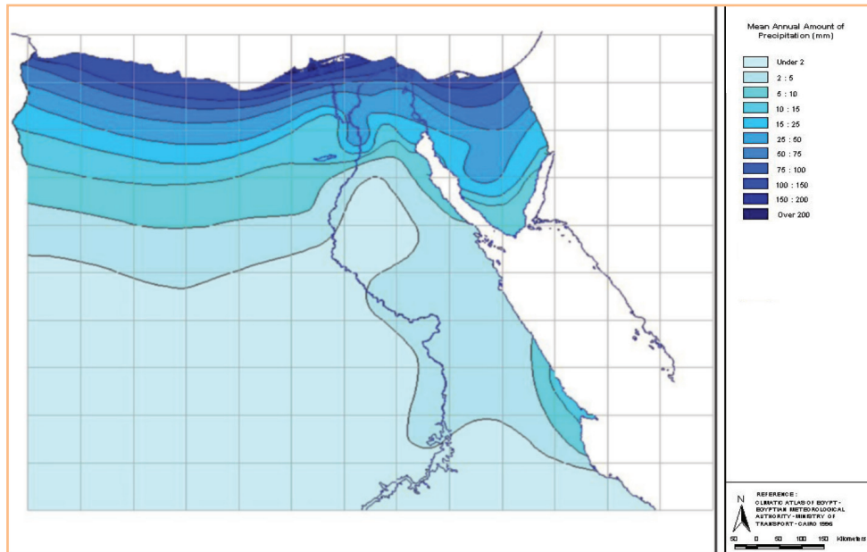
Figure (I.4): Mean annual precipitation (mm). 2
