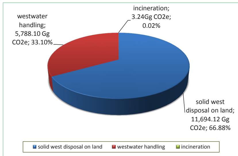
Figure (II.11): GHGs emissions and relative weight of different source categories for the waste sector, 2000.
