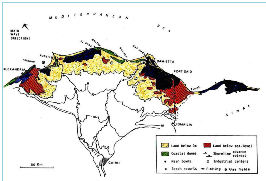
Figure (IV.5): General topography of the Nile Delta indicating areas below mean sea level (El Raey, 2009).
