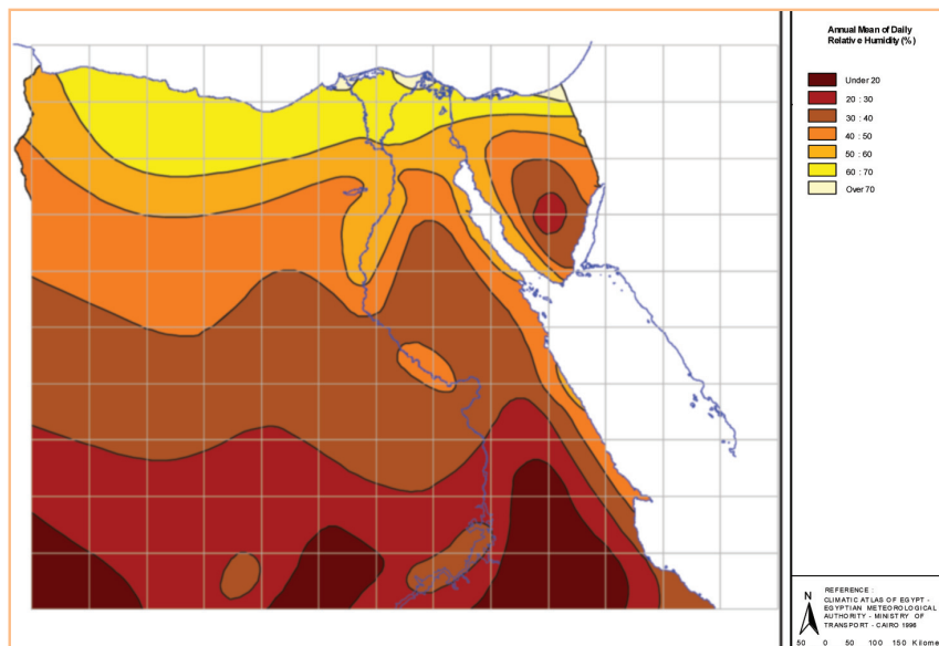
Figure (I.3): Annual mean of daily relative humidity (%). 2
