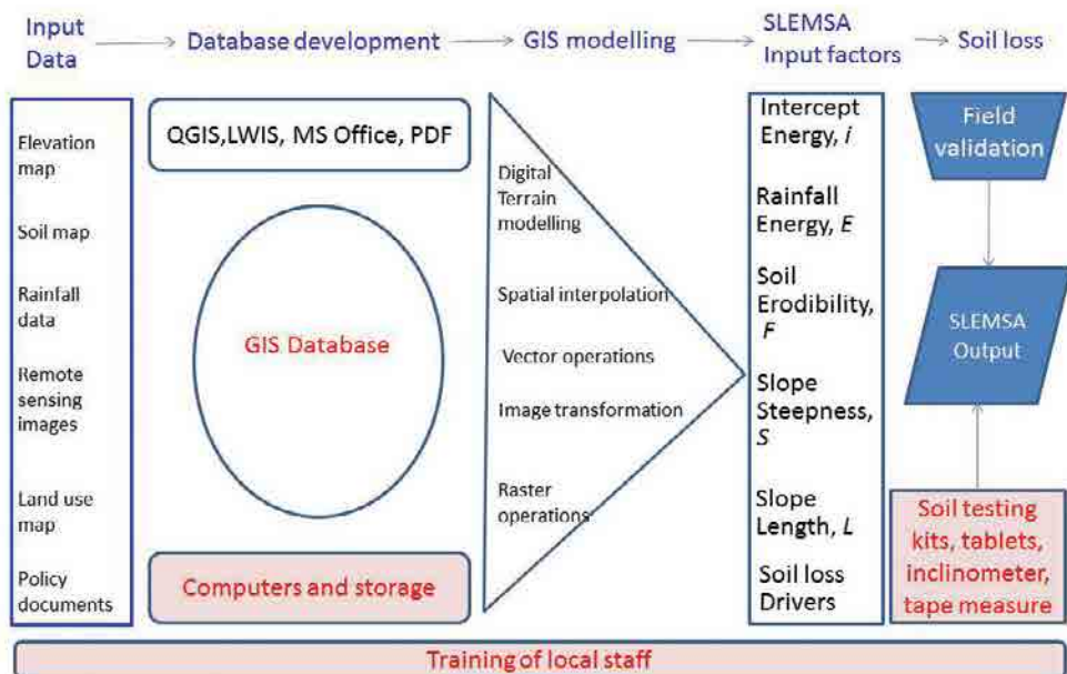
Figure 4.1: Methodological framework
