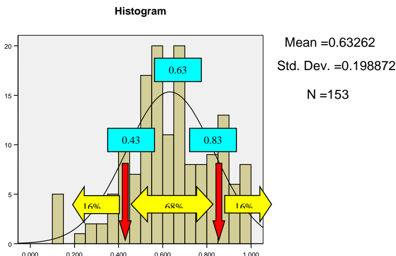
Mean: 0.63 , SD: 0.198 , N: 153 Benchmarks for Specific Electrical Energy Consumption
