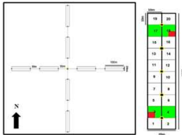
Figure 24: Design of the sampling unit applied during the pilot NFI project
