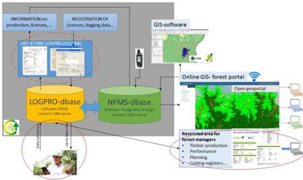
Figure 27: Monitoring framework for logging emission factors
