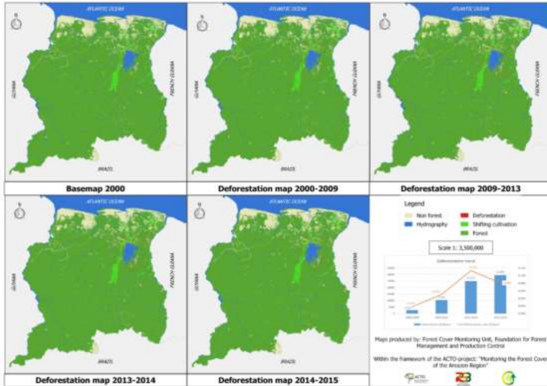
Figure 15: Suriname deforestation maps
