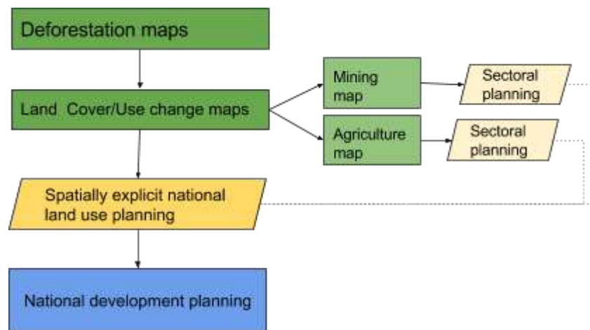
Figure 17: SLMS maps for multiple purposes
