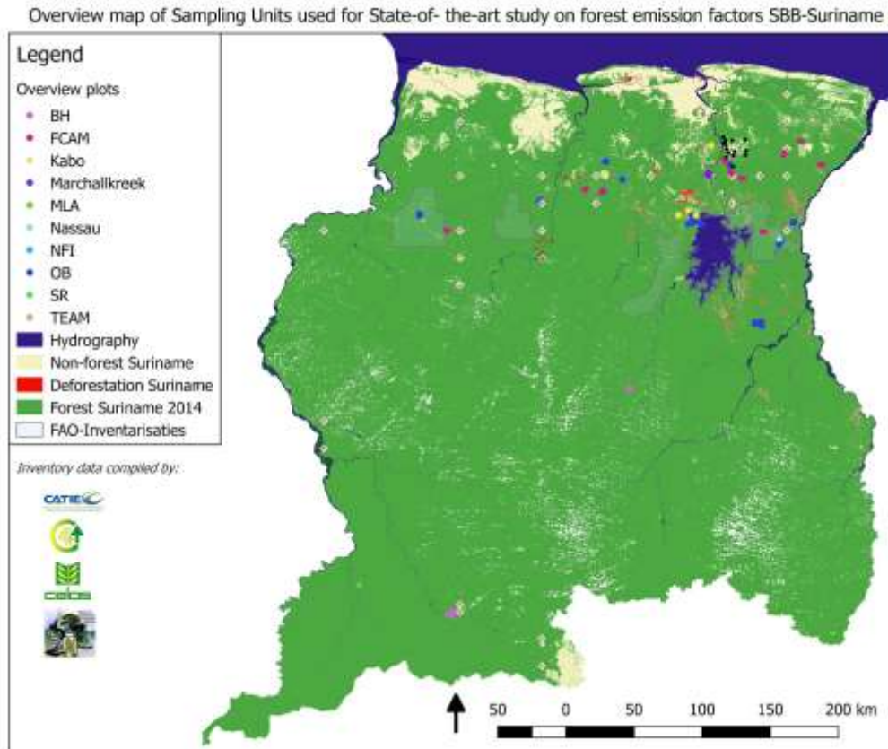
Figure 21: Overview of sampling units included in EF study
