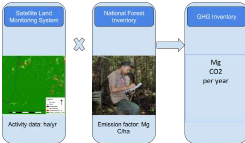
Figure 22: Integration of remote sensing and field data for reporting
