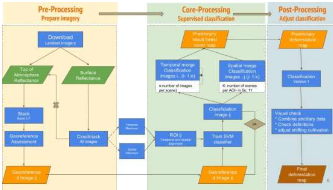
Figure 14: Methodology to produce deforestation maps
