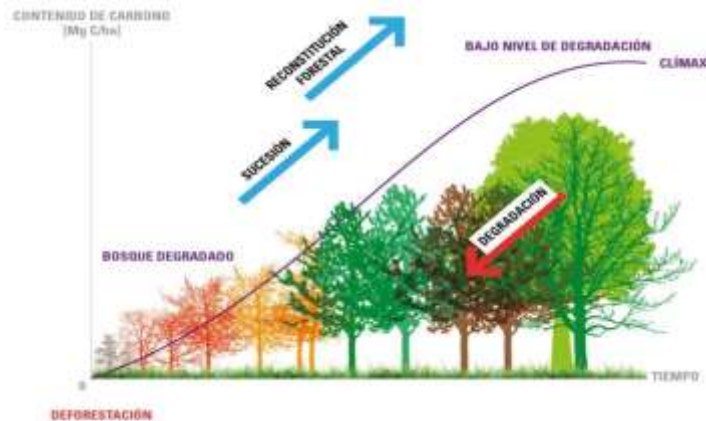
Figure 16: Visualization of forest degradation in terms of carbon loss
