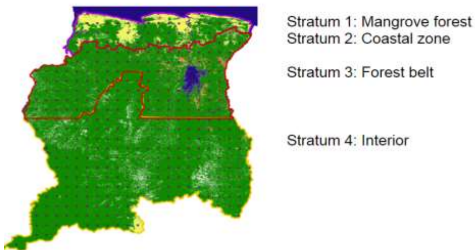
Figure 23: Stratification of Suriname
